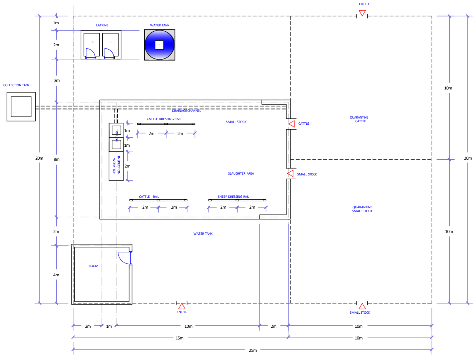
LAYOUT PLAN
